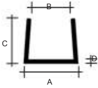
C SECTION
